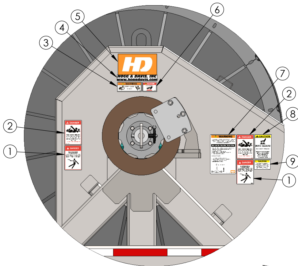
DETAIL B SCALE 1 : 12
